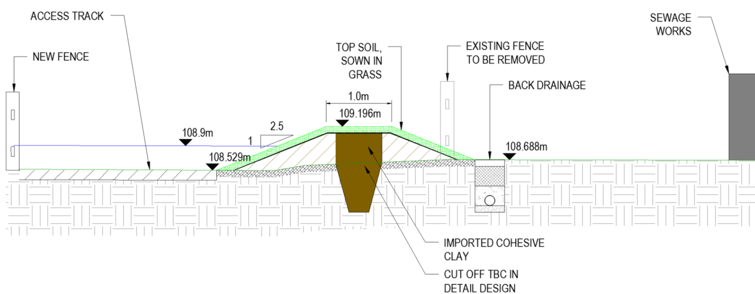
Location 2: Typical flood embankment cross section at Sewage Works*
