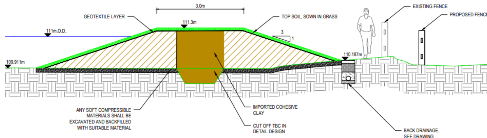
Location 1: Typical flood embankment cross section at Old Cleish Road
